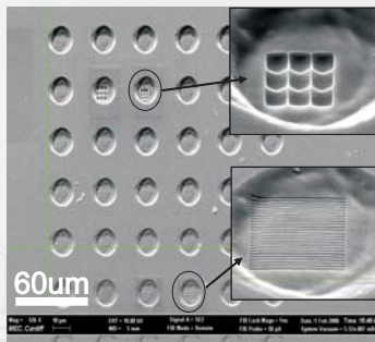
Diffraction gratings and micro lenses
